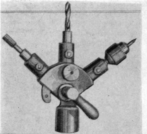
The Eisler turret attachment for engine lathes (Patent No. 1,209,650), designed in 1916 to handle drill-jig and die brushings, screws, studs and nuts, and used for recessing holes of various kinds.
